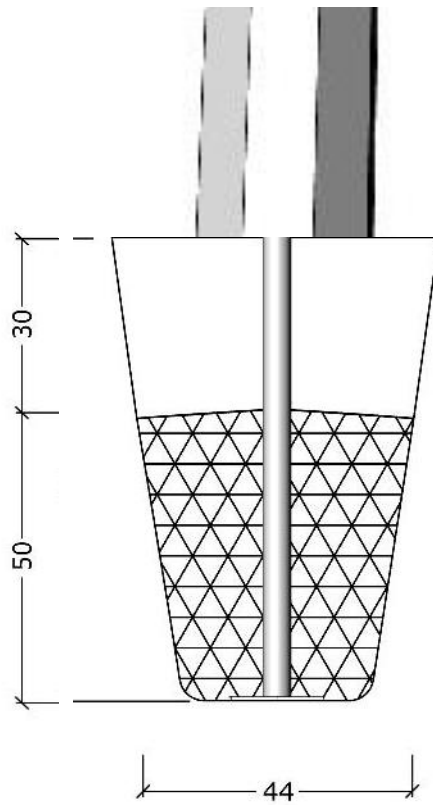
Fundering "benzinstander"
